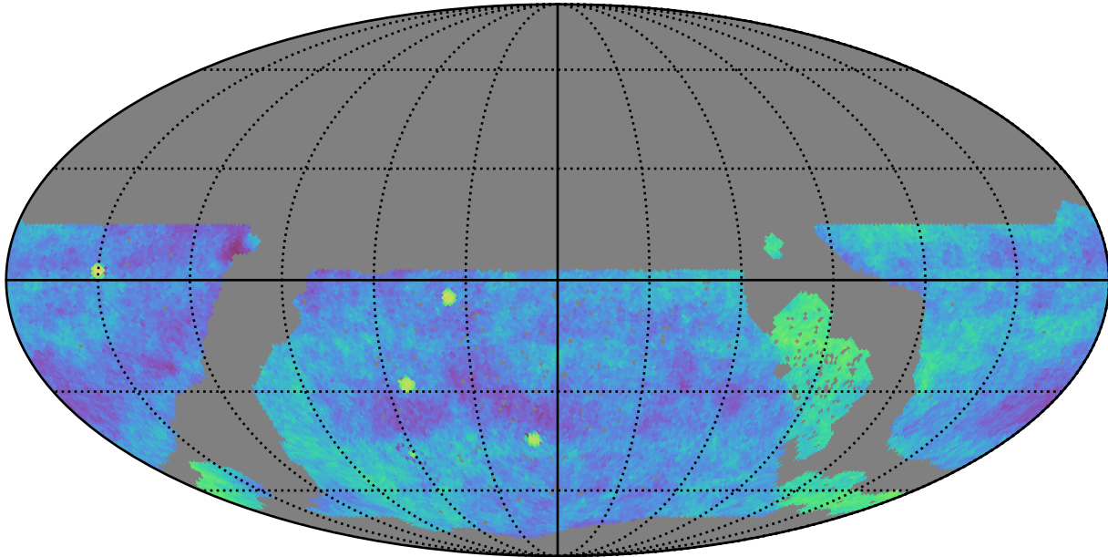
roll_uniform_early_half_mjdp0_v3.4_10yrs gri WFD: Fraction of visits in pairs (20-90 min)
