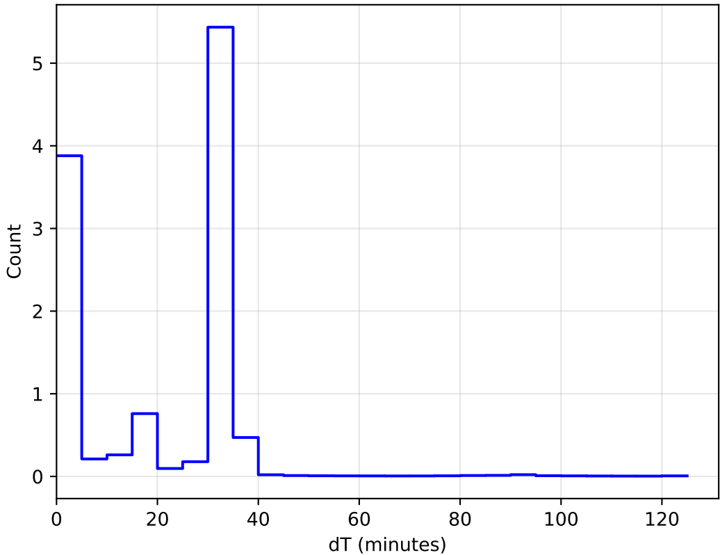
roll_uniform_early_half_mjdp0_v3.4_10yrs WFD: DeltaT Histogram 1e6
