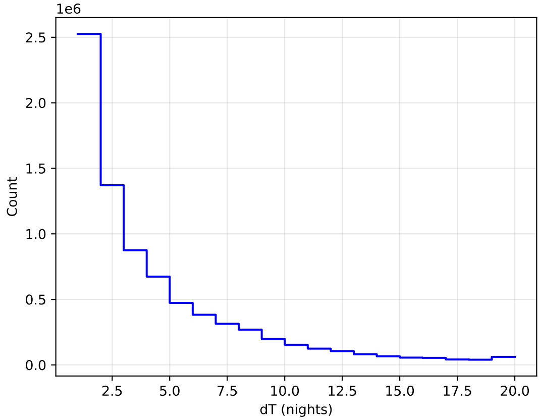
roll_uniform_early_half_mjdp0_v3.4_10yrs WFD all bands: DeltaNight Histogram
