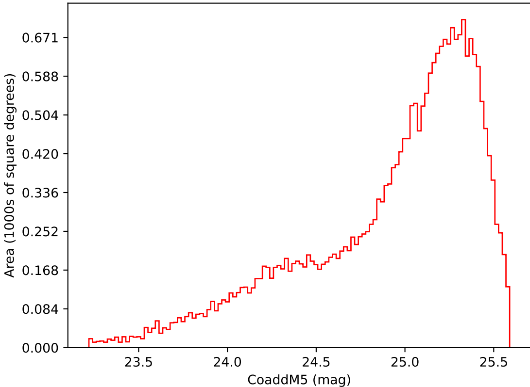
roll_uniform_early_half_mjdp0_v3.4_10yrs Yr 3-4 i band: CoaddM5
