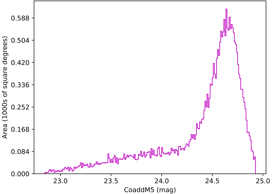
roll_uniform_early_half_mjdp0_v3.4_10yrs Yr 1 z band: CoaddM5
