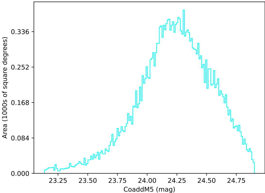
roll_uniform_early_half_mjdp0_v3.4_10yrs Yr 1 u band: CoaddM5
