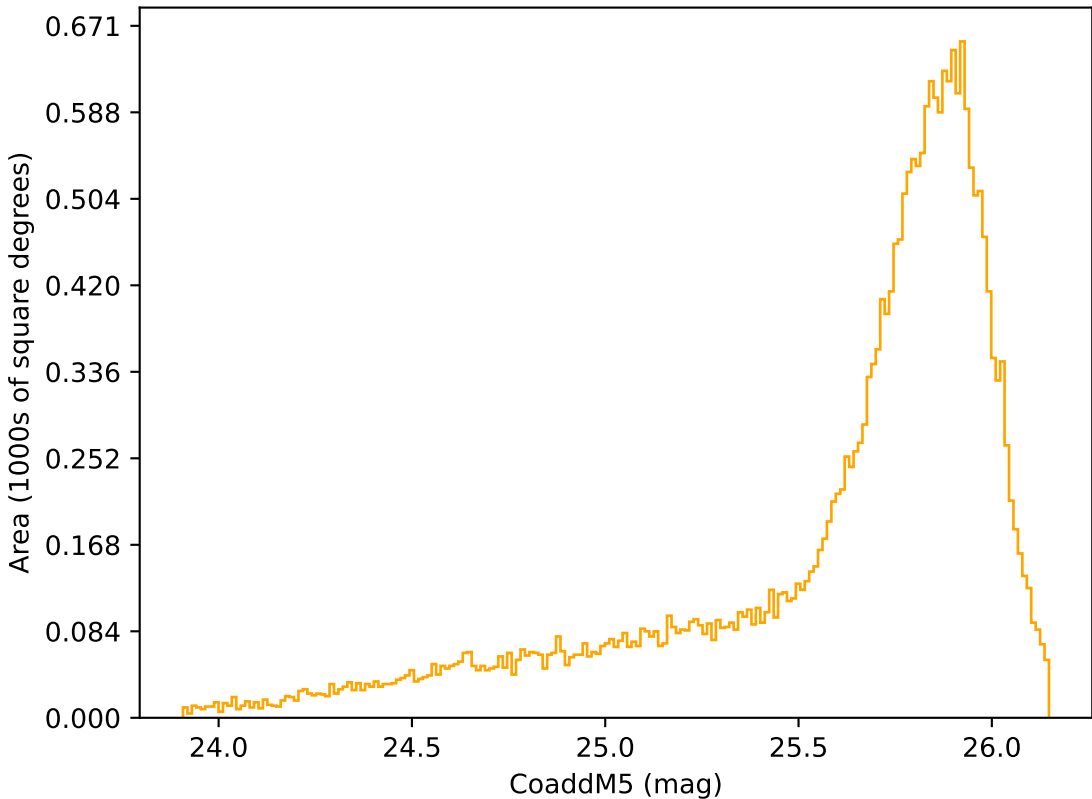
roll_uniform_early_half_mjdp0_v3.4_10yrs Yr 1 r band: CoaddM5
