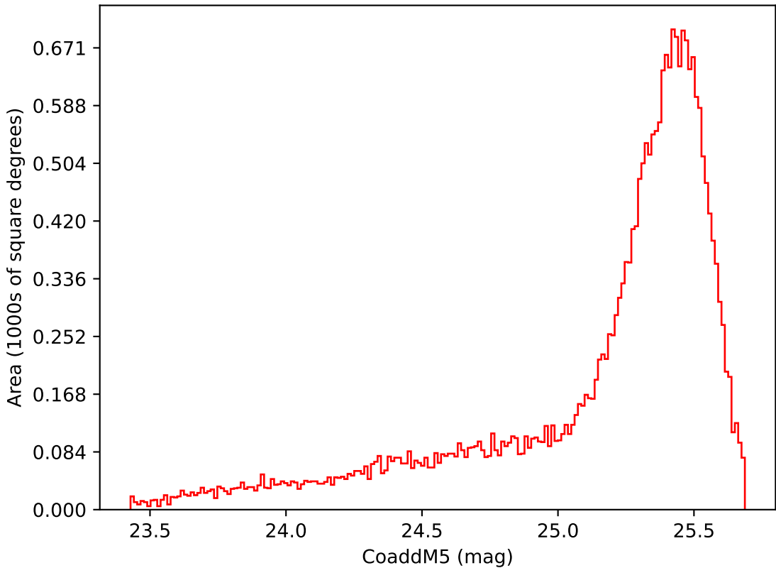
roll_uniform_early_half_mjdp0_v3.4_10yrs Yr 1 i band: CoaddM5
