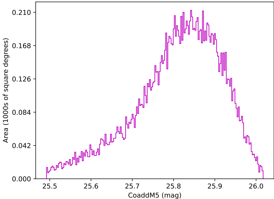
roll_uniform_early_half_mjdp0_v3.4_10yrs WFD z band: CoaddM5
