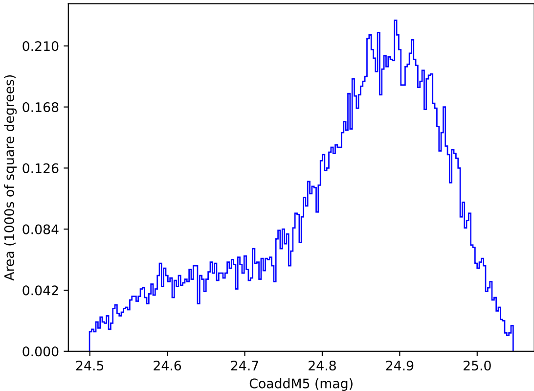
roll_uniform_early_half_mjdp0_v3.4_10yrs WFD y band: CoaddM5
