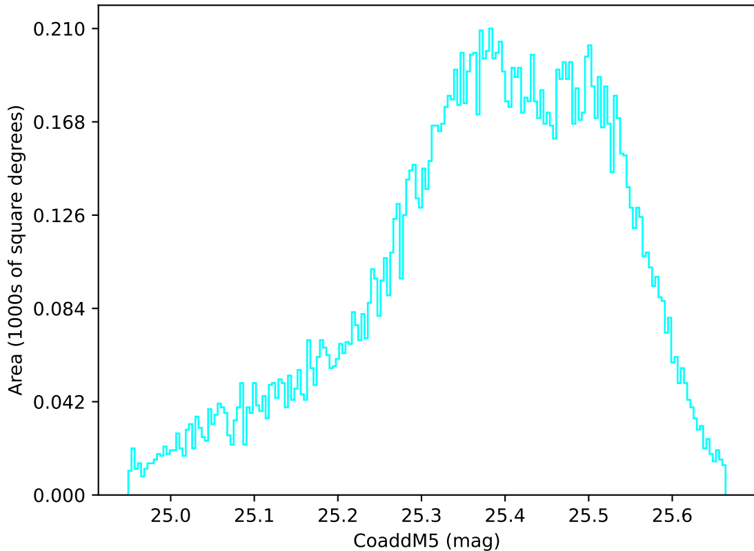
roll_uniform_early_half_mjdp0_v3.4_10yrs WFD u band: CoaddM5
