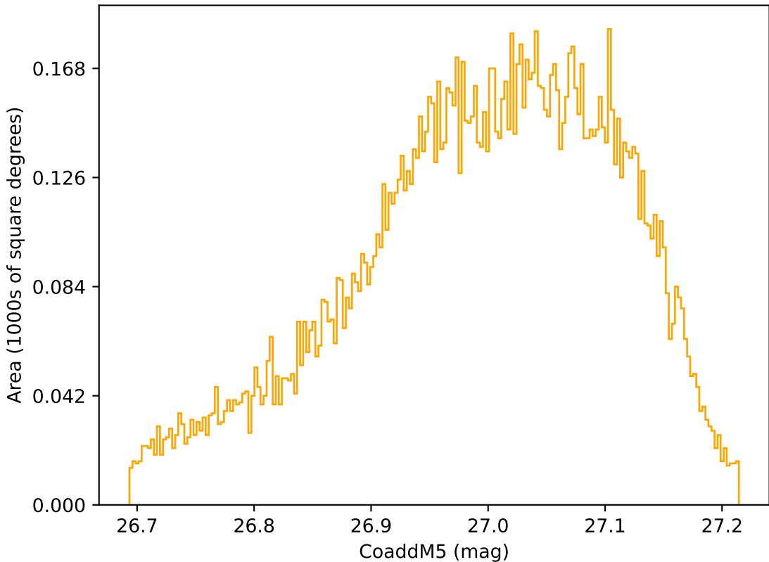
roll_uniform_early_half_mjdp0_v3.4_10yrs WFD r band: CoaddM5
