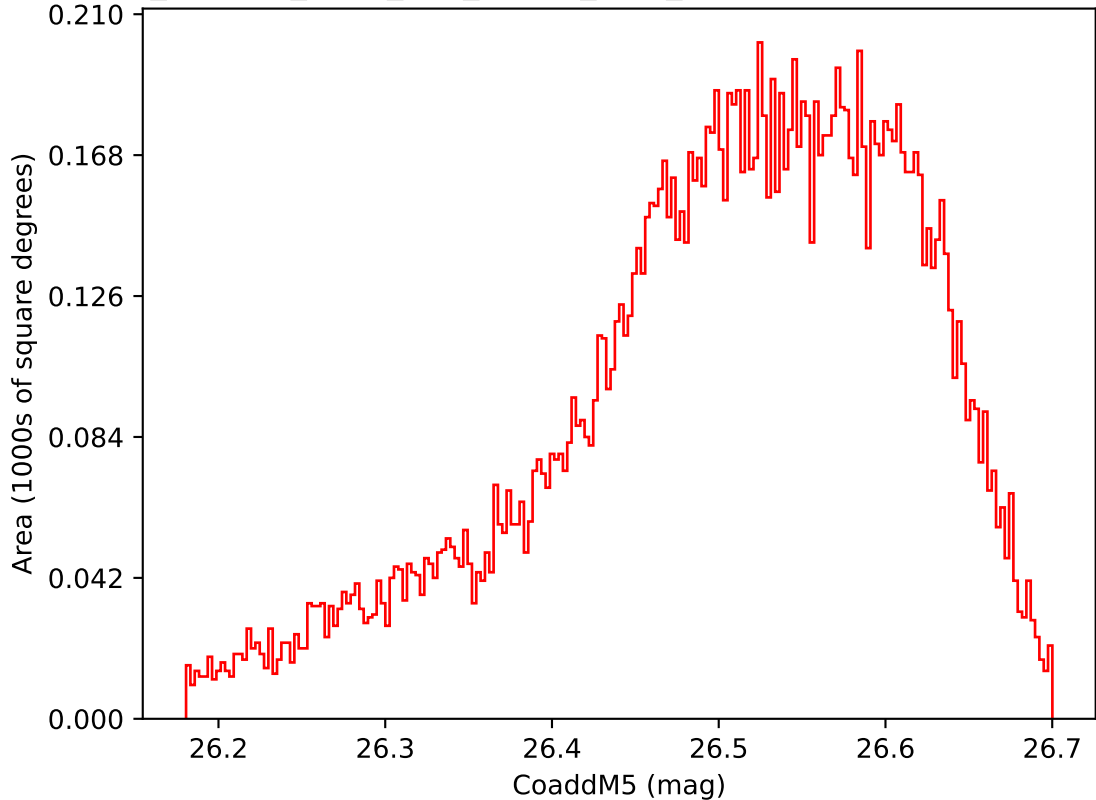
roll_uniform_early_half_mjdp0_v3.4_10yrs WFD i band: CoaddM5
