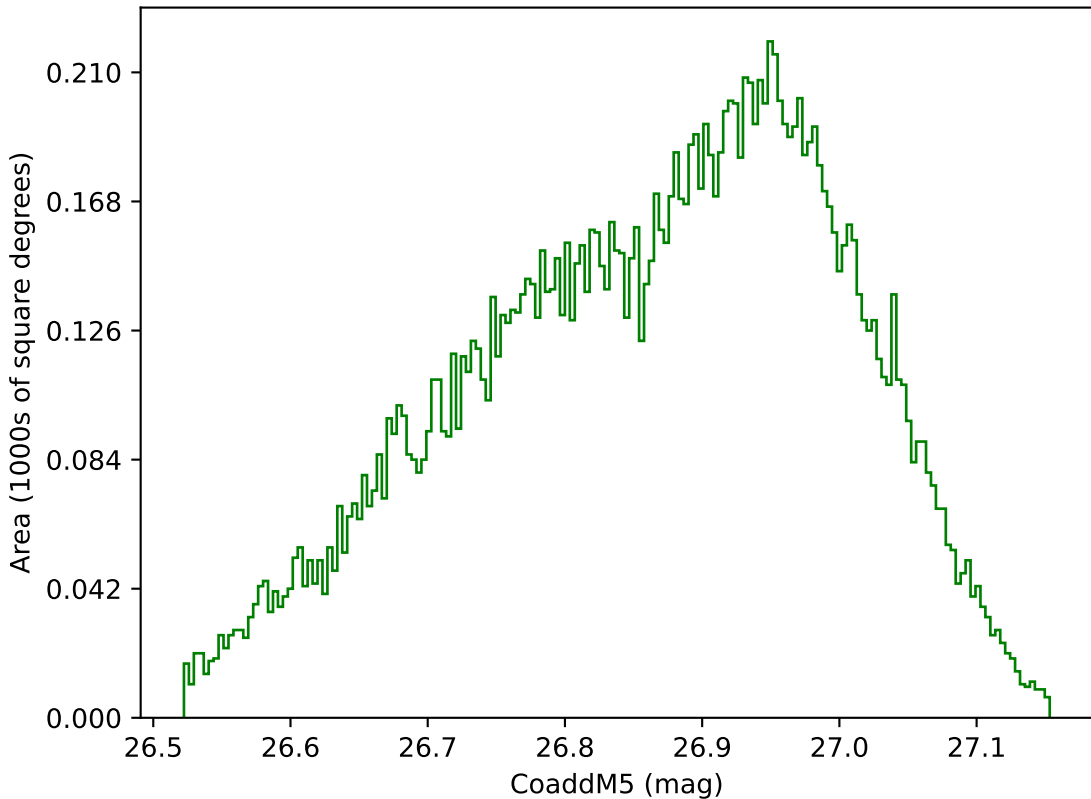
roll_uniform_early_half_mjdp0_v3.4_10yrs WFD g band: CoaddM5
