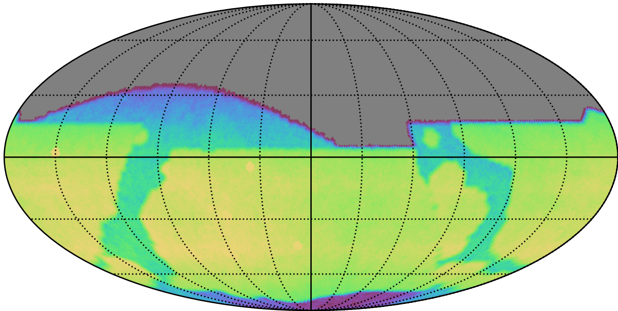
roll_uniform_early_half_mjdp0_v3.4_10yrs All sky r band: CoaddM5
