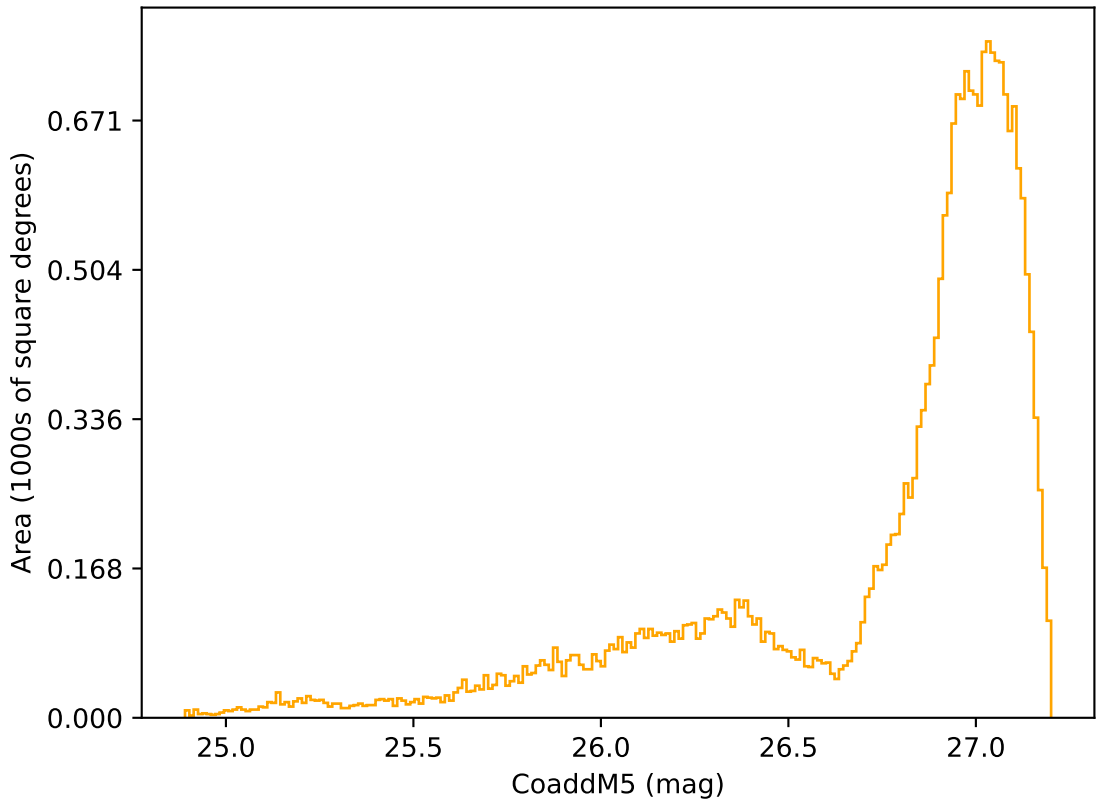
roll_uniform_early_half_mjdp0_v3.4_10yrs All sky r band: CoaddM5
