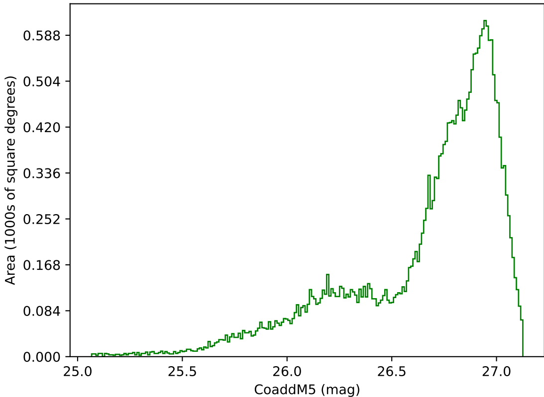
roll_uniform_early_half_mjdp0_v3.4_10yrs All sky g band: CoaddM5
