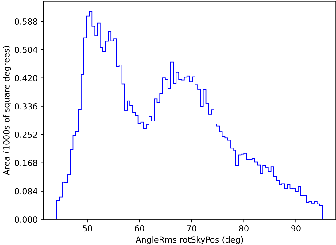
roll_uniform_early_half_mjdp0_v3.4_10yrs All sky all bands: AngleRms rotSkyPos
