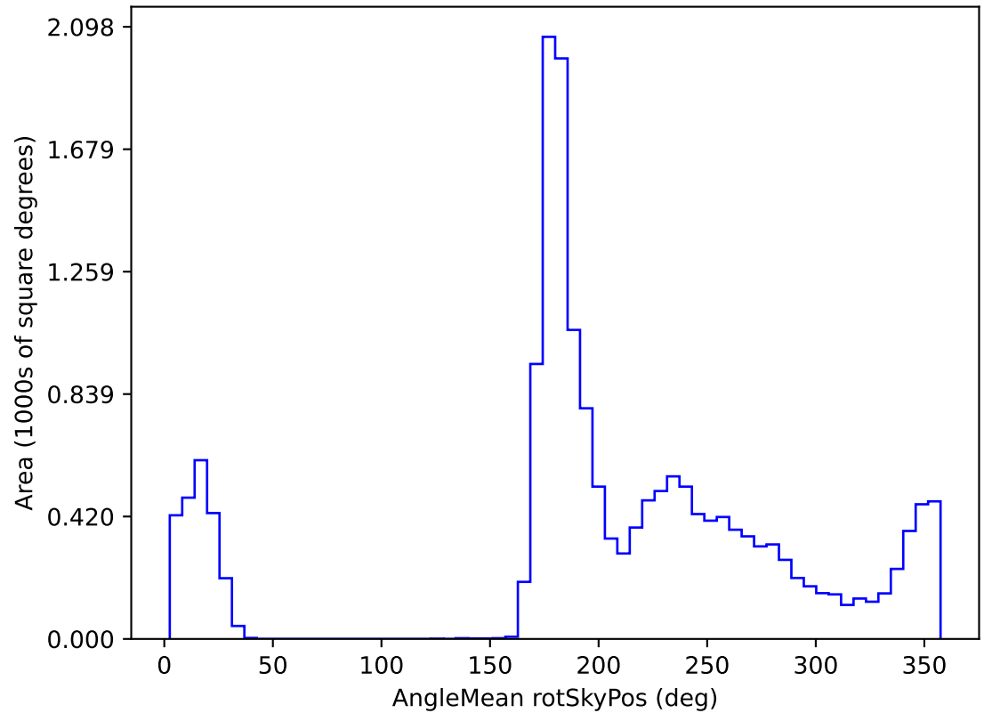
roll_uniform_early_half_mjdp0_v3.4_10yrs WFD i band: AngleMean rotSkyPos
