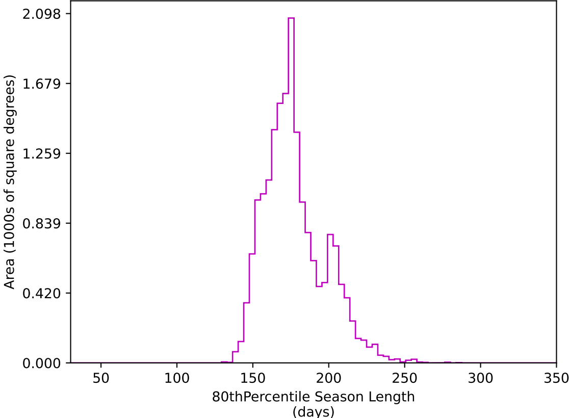
roll_uniform_early_half_mjdp0_v3.4_10yrs WFD z band: 80thPercentile Season Length
