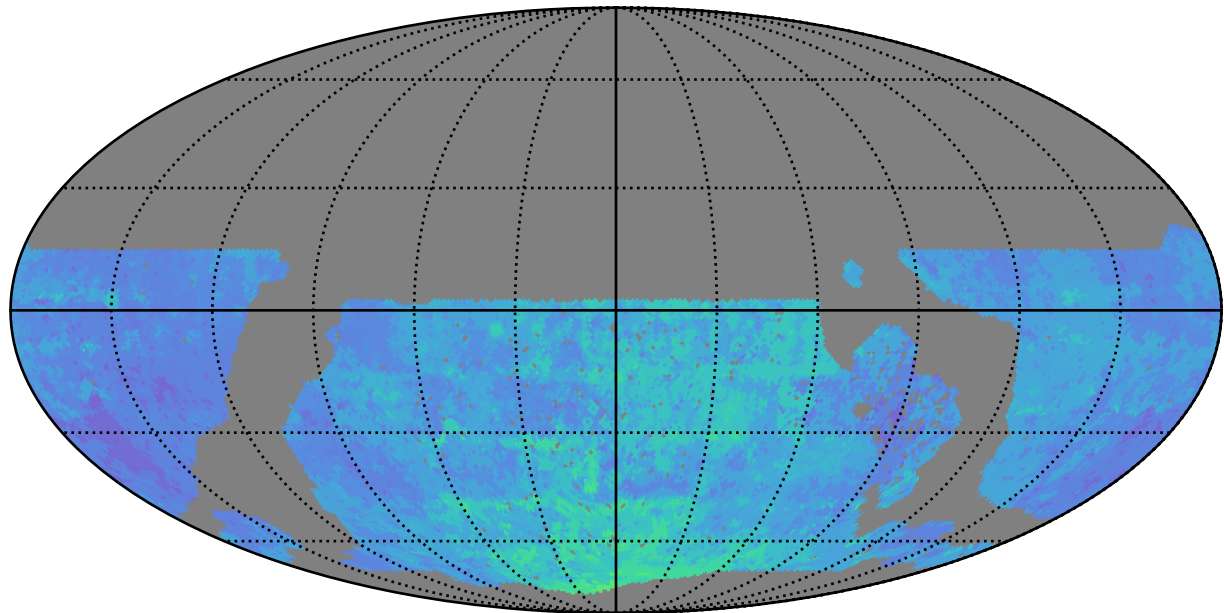
roll_uniform_early_half_mjdp0_v3.4_10yrs WFD y band: 80thPercentile Season Length
