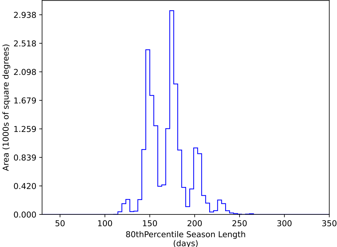
roll_uniform_early_half_mjdp0_v3.4_10yrs WFD y band: 80thPercentile Season Length
