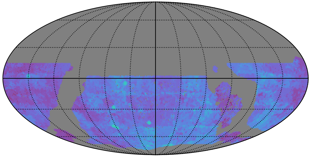
roll_uniform_early_half_mjdp0_v3.4_10yrs WFD u band: 80thPercentile Season Length
