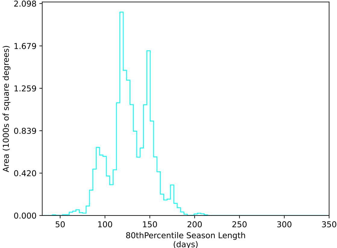
roll_uniform_early_half_mjdp0_v3.4_10yrs WFD u band: 80thPercentile Season Length
