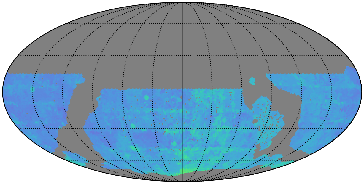
roll_uniform_early_half_mjdp0_v3.4_10yrs WFD r band: 80thPercentile Season Length
