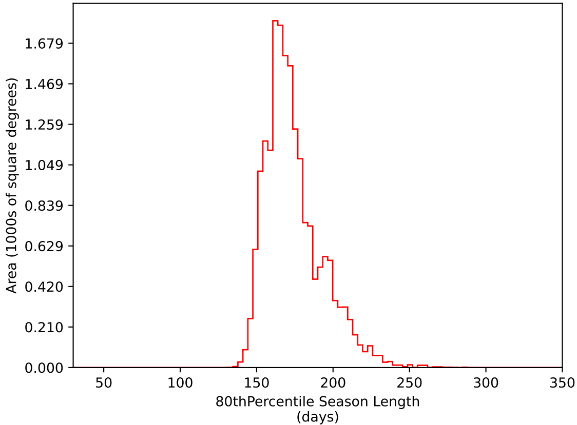
roll_uniform_early_half_mjdp0_v3.4_10yrs WFD i band: 80thPercentile Season Length
