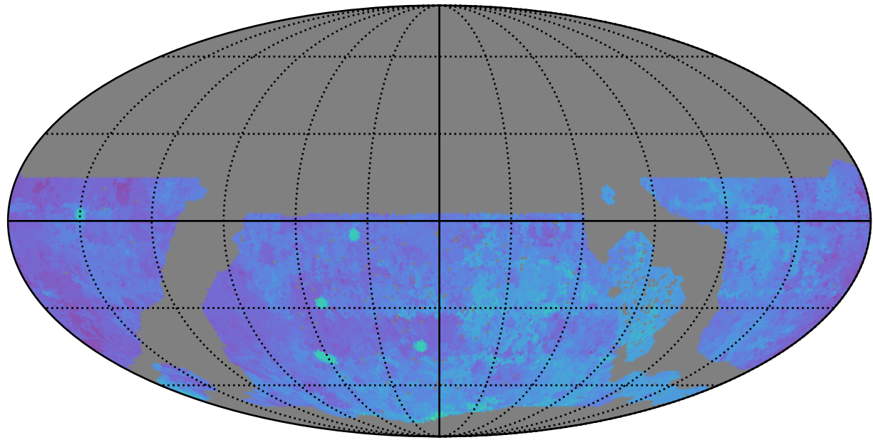
roll_uniform_early_half_mjdp0_v3.4_10yrs WFD g band: 80thPercentile Season Length
