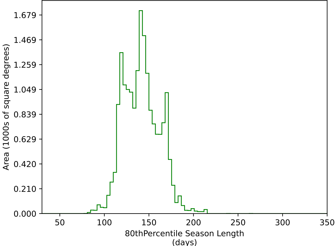
roll_uniform_early_half_mjdp0_v3.4_10yrs WFD g band: 80thPercentile Season Length
