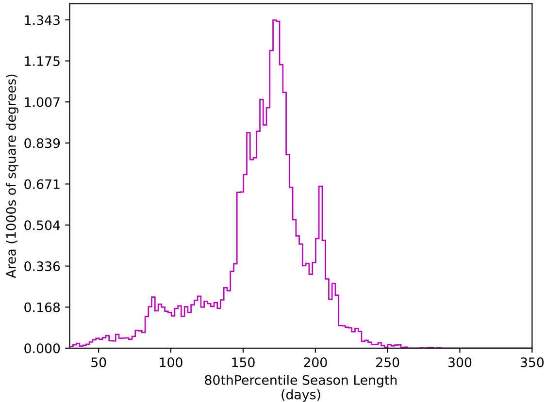
roll_uniform_early_half_mjdp0_v3.4_10yrs All sky z band: 80thPercentile Season Length
