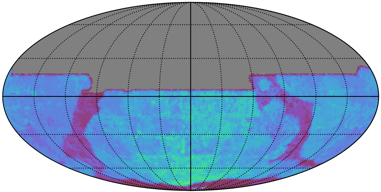
roll_uniform_early_half_mjdp0_v3.4_10yrs All sky y band: 80thPercentile Season Length
