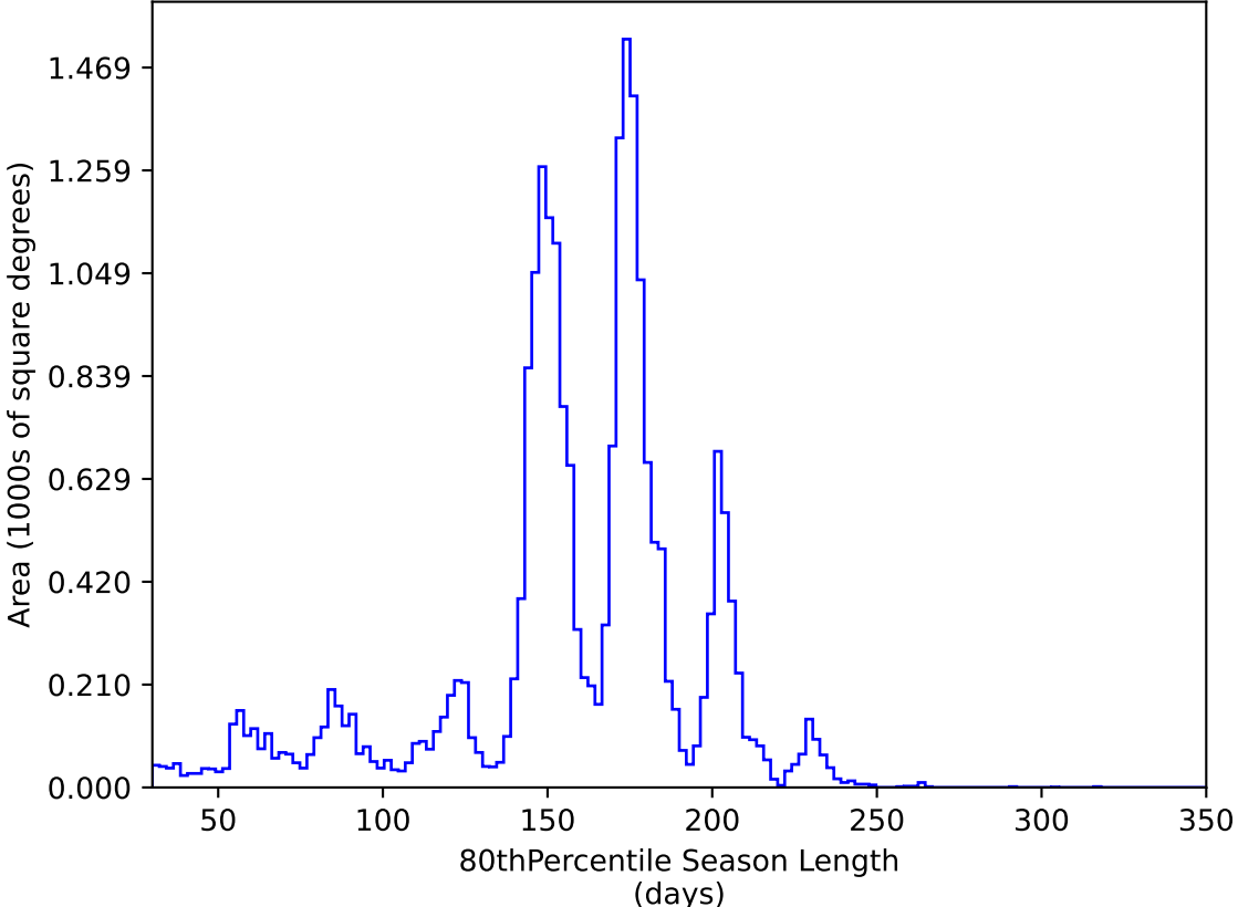
roll_uniform_early_half_mjdp0_v3.4_10yrs All sky y band: 80thPercentile Season Length
