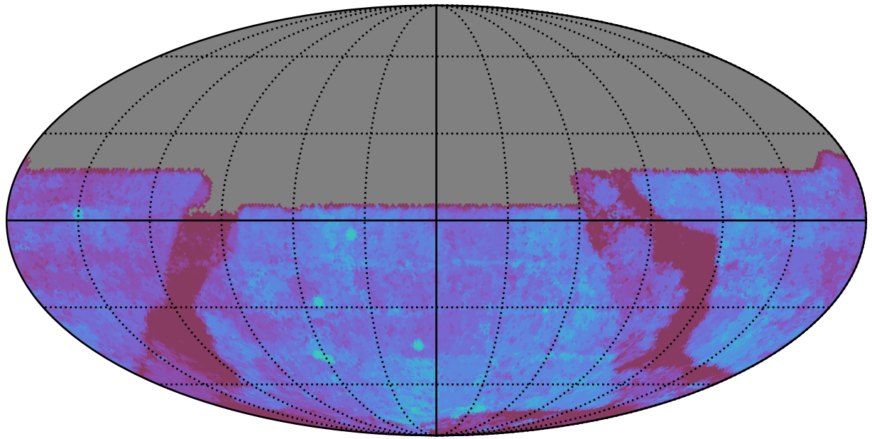
roll_uniform_early_half_mjdp0_v3.4_10yrs All sky u band: 80thPercentile Season Length
