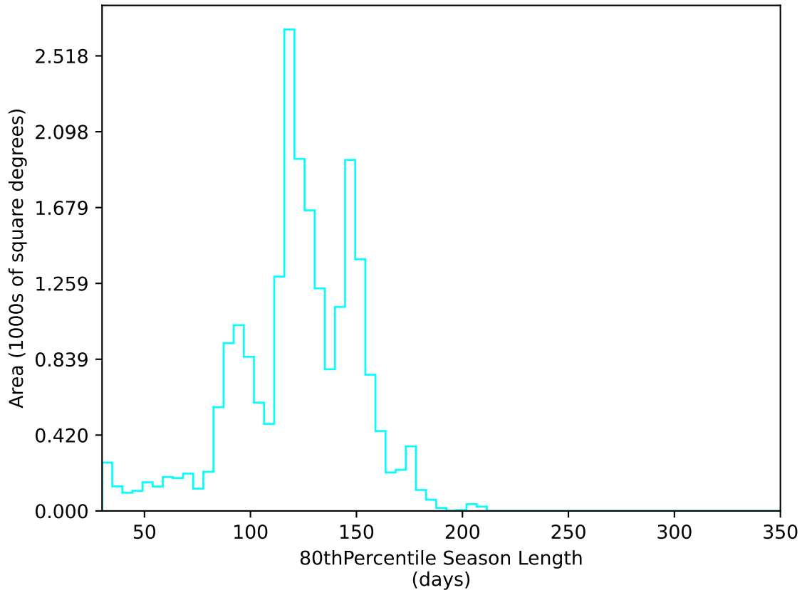
roll_uniform_early_half_mjdp0_v3.4_10yrs All sky u band: 80thPercentile Season Length
