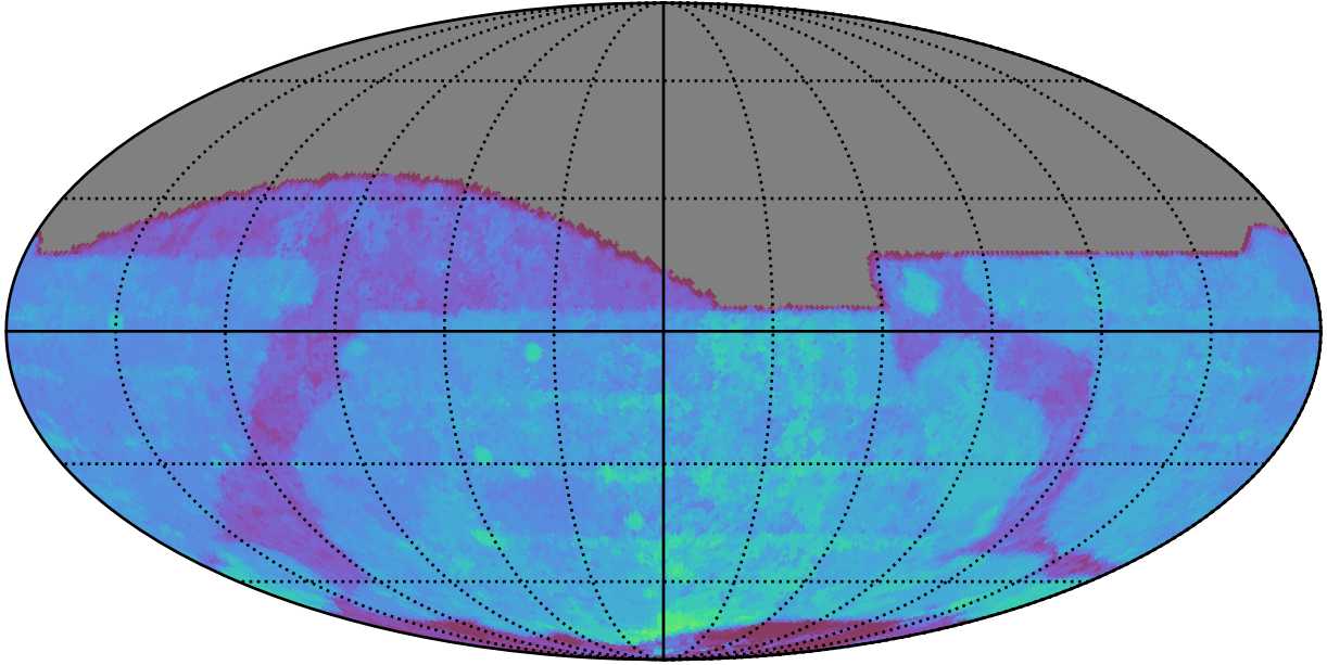
roll_uniform_early_half_mjdp0_v3.4_10yrs All sky r band: 80thPercentile Season Length
