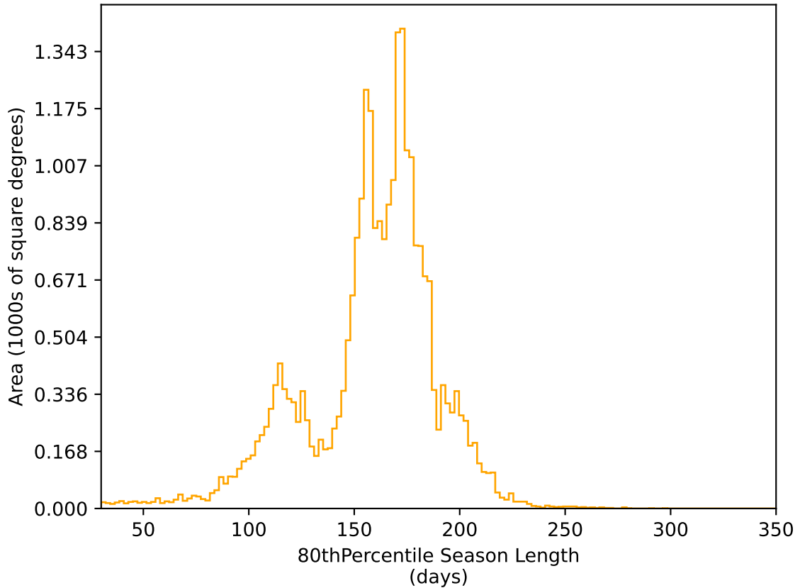
roll_uniform_early_half_mjdp0_v3.4_10yrs All sky r band: 80thPercentile Season Length
