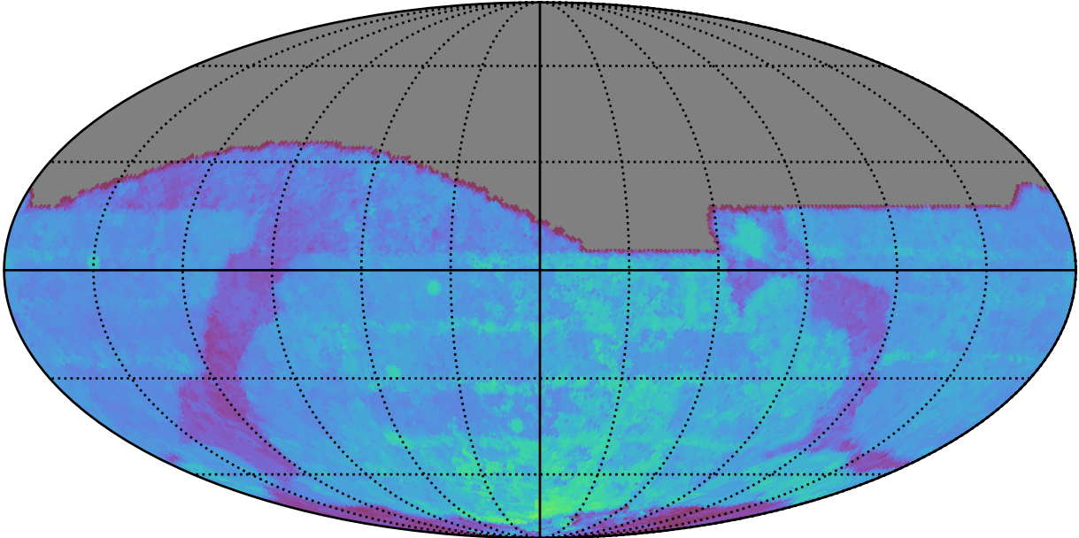
roll_uniform_early_half_mjdp0_v3.4_10yrs All sky i band: 80thPercentile Season Length
