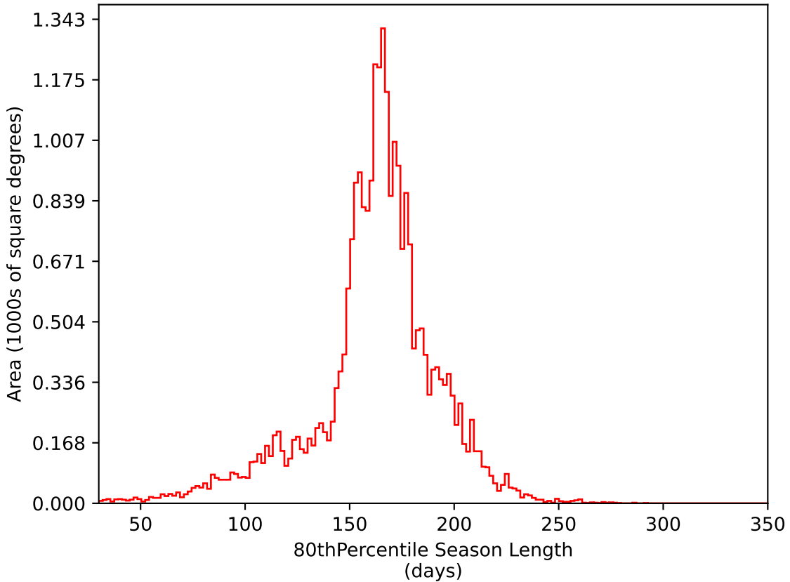
roll_uniform_early_half_mjdp0_v3.4_10yrs All sky i band: 80thPercentile Season Length
