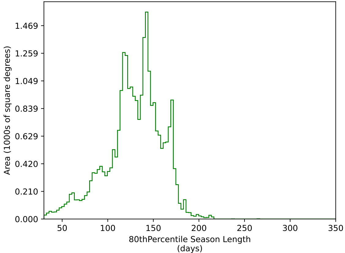
roll_uniform_early_half_mjdp0_v3.4_10yrs All sky g band: 80thPercentile Season Length
