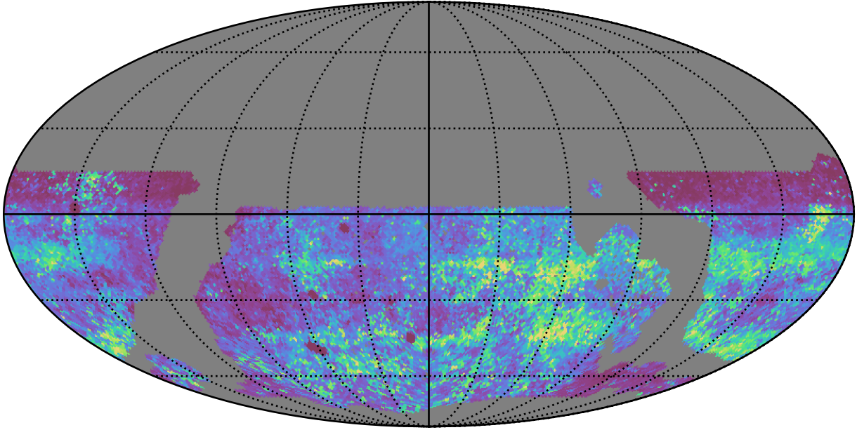
roll_uniform_early_half_mjdp0_v3.4_10yrs WFD zy bands: 75th Percentile Intranight Timespan
