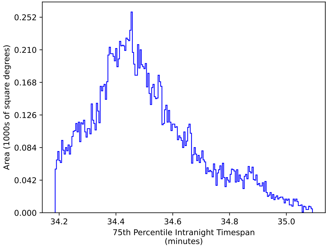
roll_uniform_early_half_mjdp0_v3.4_10yrs WFD zy bands: 75th Percentile Intranight Timespan
