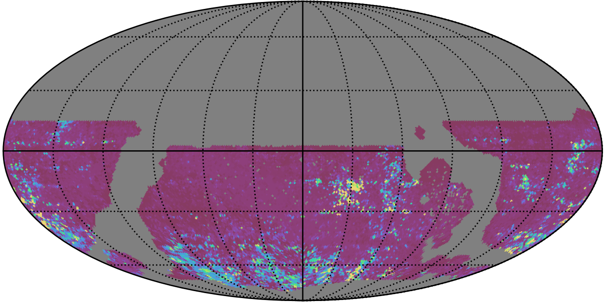
roll_uniform_early_half_mjdp0_v3.4_10yrs WFD z band: 75th Percentile Intranight Timespan
