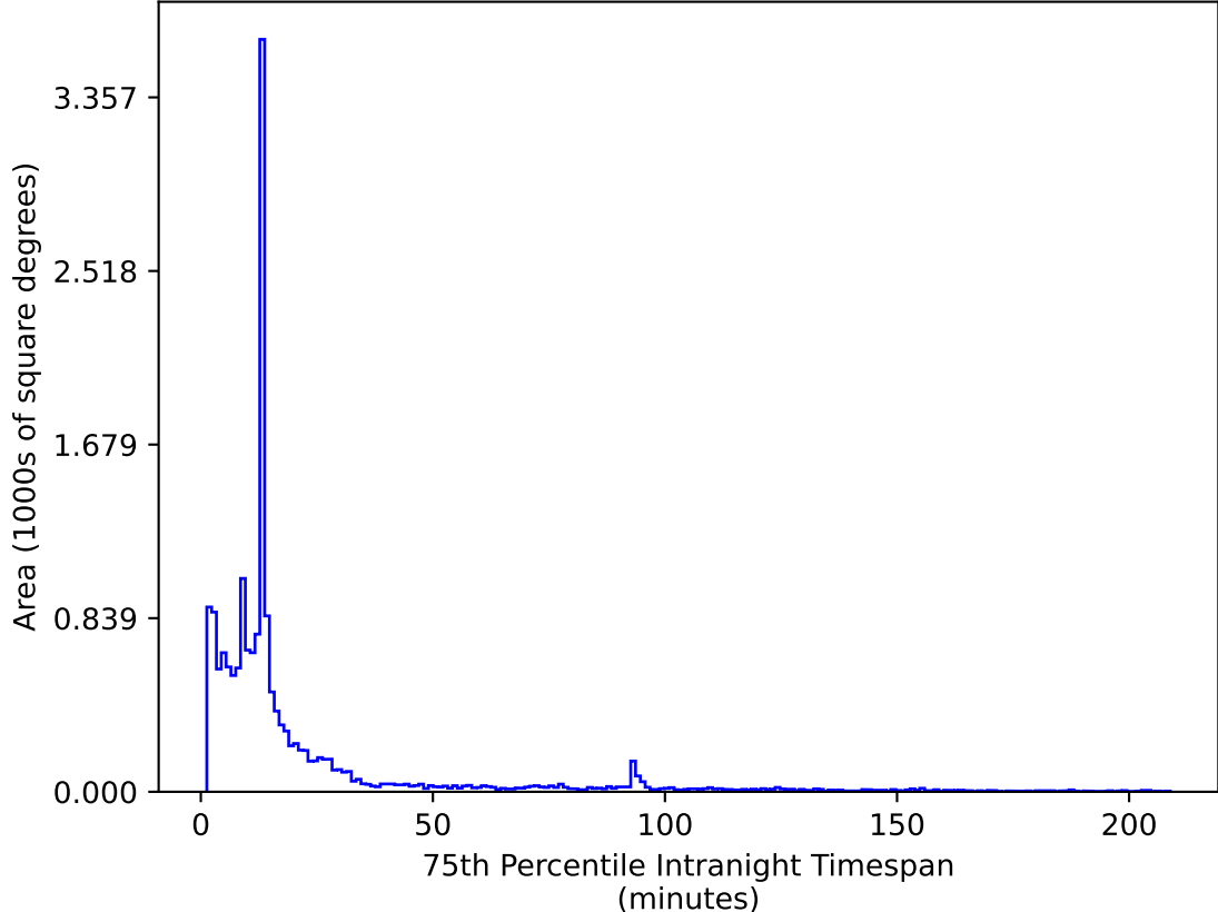
roll_uniform_early_half_mjdp0_v3.4_10yrs WFD z band: 75th Percentile Intranight Timespan
