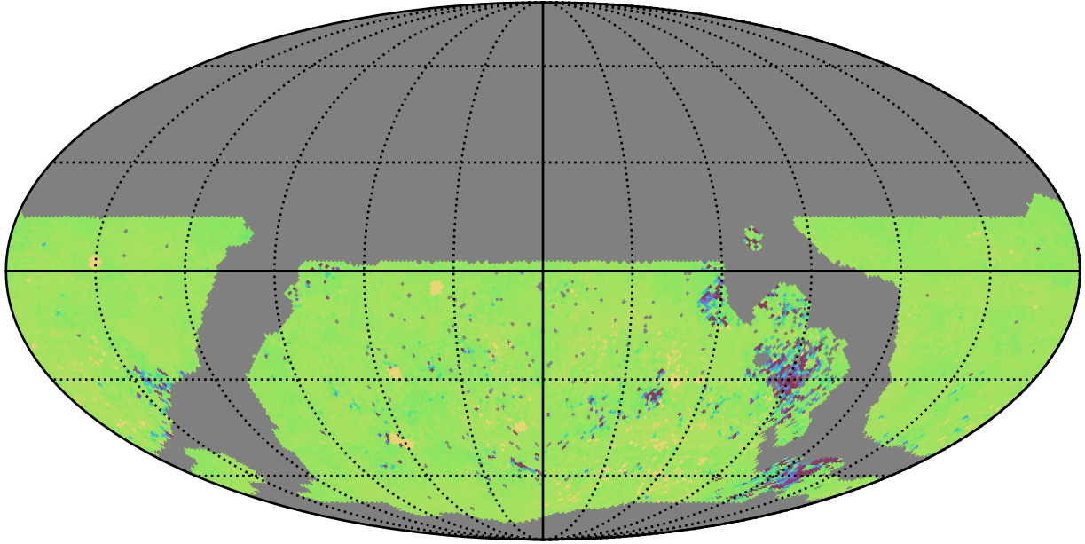
roll_uniform_early_half_mjdp0_v3.4_10yrs WFD ug bands: 75th Percentile Intranight Timespan
