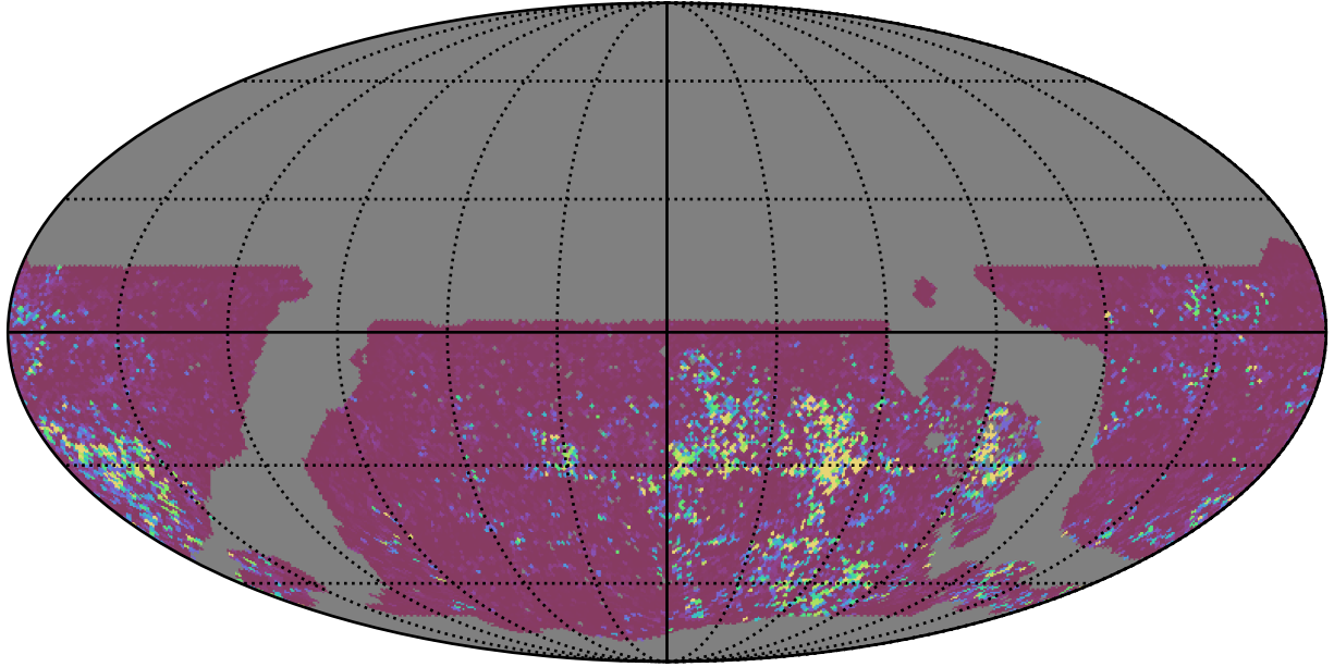
roll_uniform_early_half_mjdp0_v3.4_10yrs WFD u band: 75th Percentile Intranight Timespan
