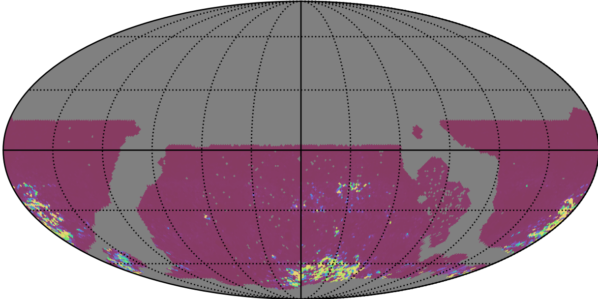
roll_uniform_early_half_mjdp0_v3.4_10yrs WFD ri bands: 75th Percentile Intranight Timespan
