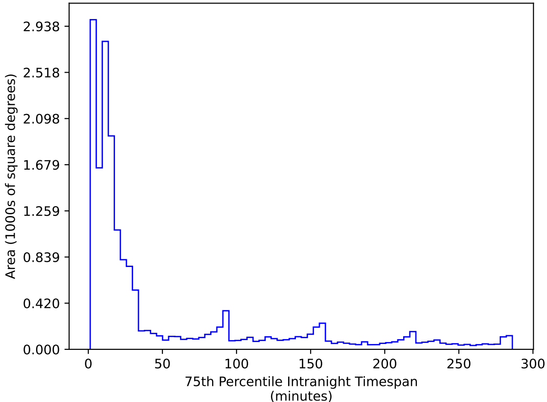
roll_uniform_early_half_mjdp0_v3.4_10yrs WFD r band: 75th Percentile Intranight Timespan
