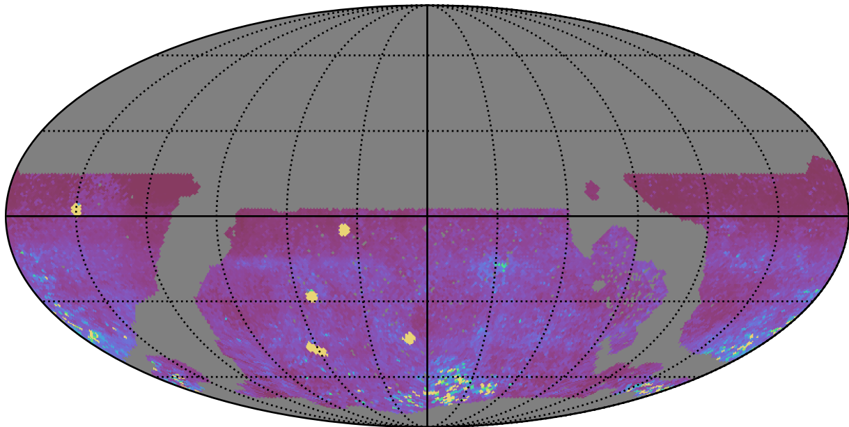
roll_uniform_early_half_mjdp0_v3.4_10yrs WFD iz bands: 75th Percentile Intranight Timespan
