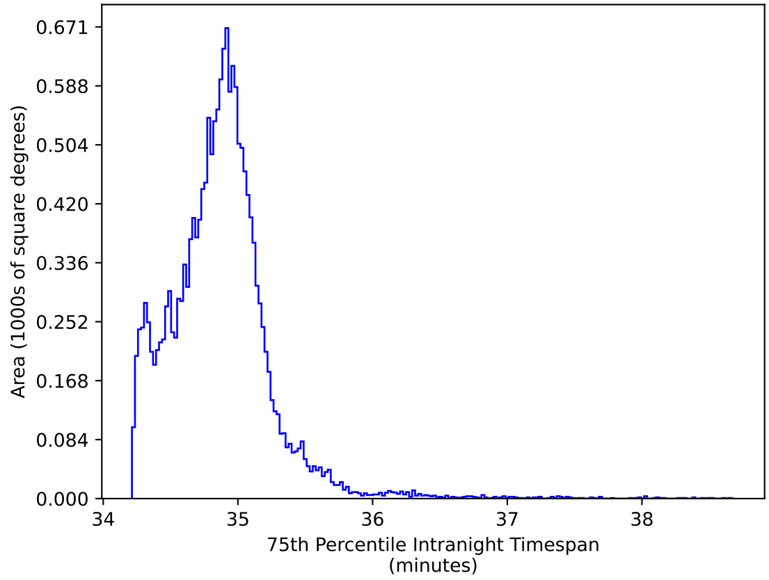
roll_uniform_early_half_mjdp0_v3.4_10yrs WFD iz bands: 75th Percentile Intranight Timespan
