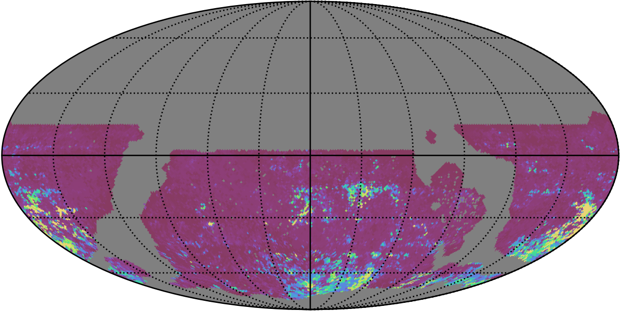
roll_uniform_early_half_mjdp0_v3.4_10yrs WFD i band: 75th Percentile Intranight Timespan
