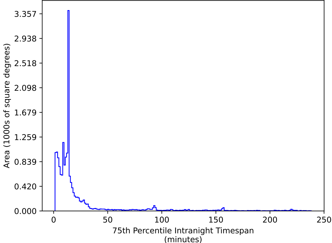
roll_uniform_early_half_mjdp0_v3.4_10yrs WFD i band: 75th Percentile Intranight Timespan
